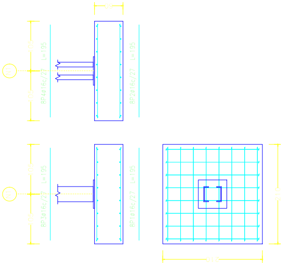
Fig. 1 Dimensiones Placa = 400x600x25 mm (S275 (UNE-EN 10025-2)) Perno = 8x20 mm B 400 S, f_y = 1.15 Espesor placa base = 25 mm
